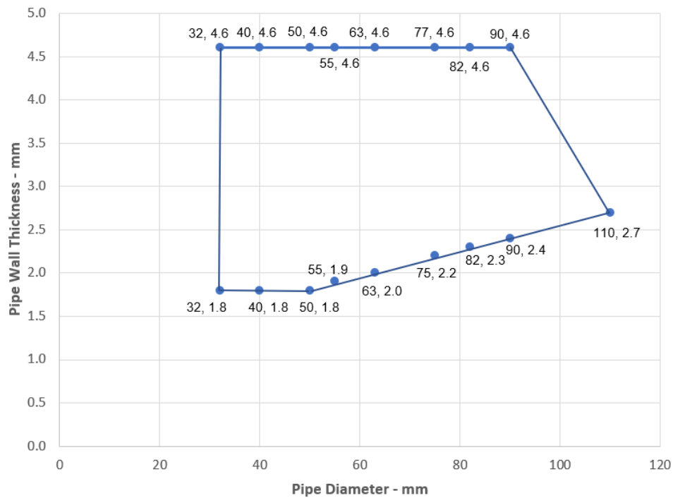
PP Pipes 32-110 / 50 mm Collar - C/C
