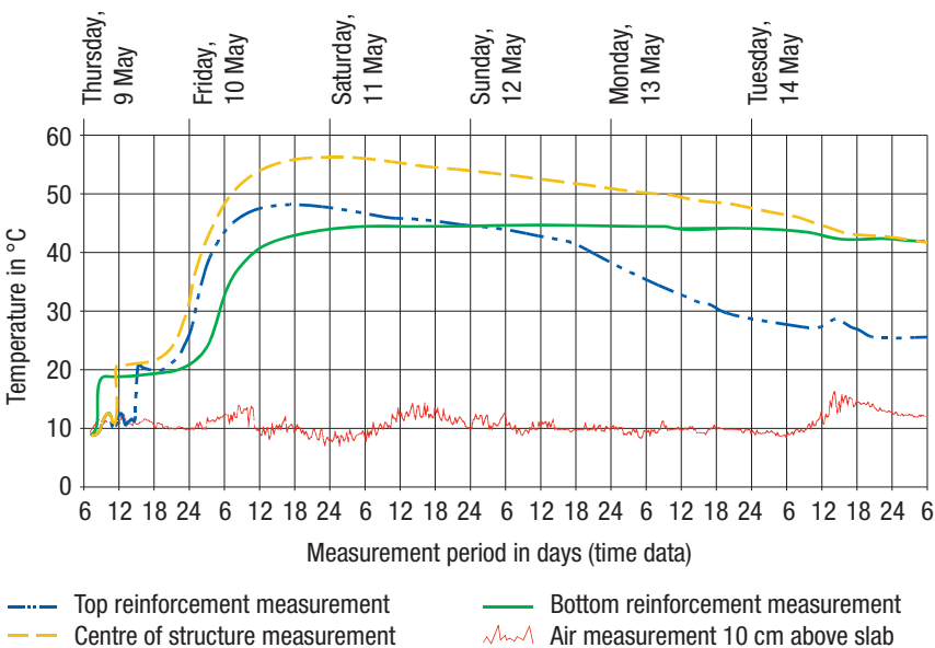
Fig. 6.5.1: Measurement of hydration heat in a 160 cm thick ground slab in three levels
