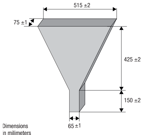
Fig. 5.2.9: V-Funnel
