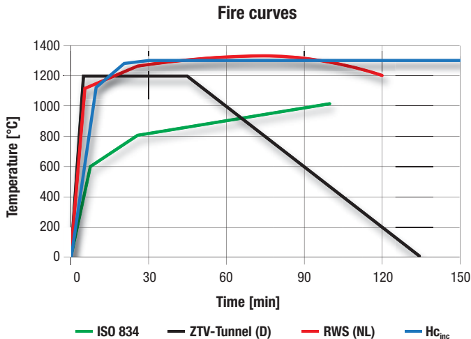
Fig. 7.6.1: Temperature-time curves of various design fires based on different regulations
