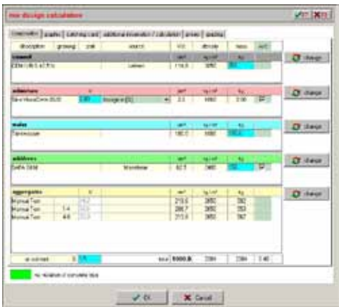
Fig. 4.3.3: Mix design calculation with change buttons for database material selection
