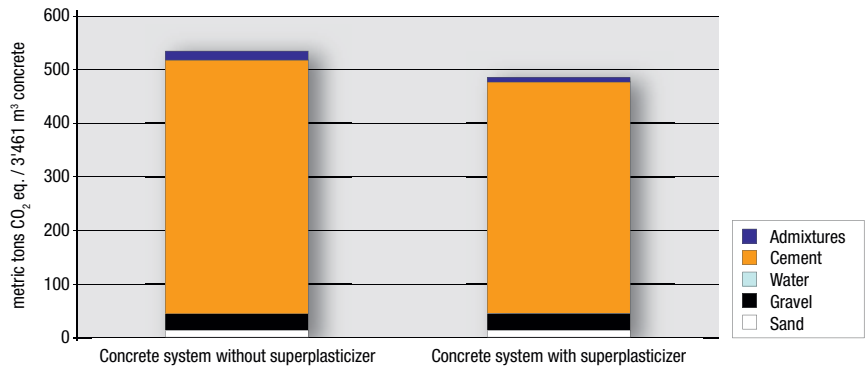
Fig. 2.2.3: Global Warming Potential with and without Sika® ViscoCrete®
