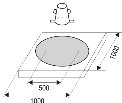
Fig. 5.2.7: Slump-flow test
