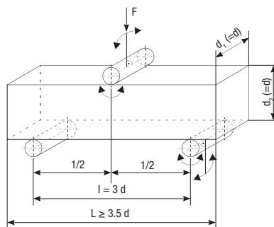
Fig. 7.10.2: Central load transfer
