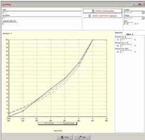
Fig. 4.3.2: Design and calculation of combined aggregated grading curve
