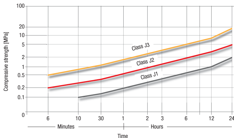
Fig. 6.9.1: Shotcrete early strength classes according to EN 14487-1
